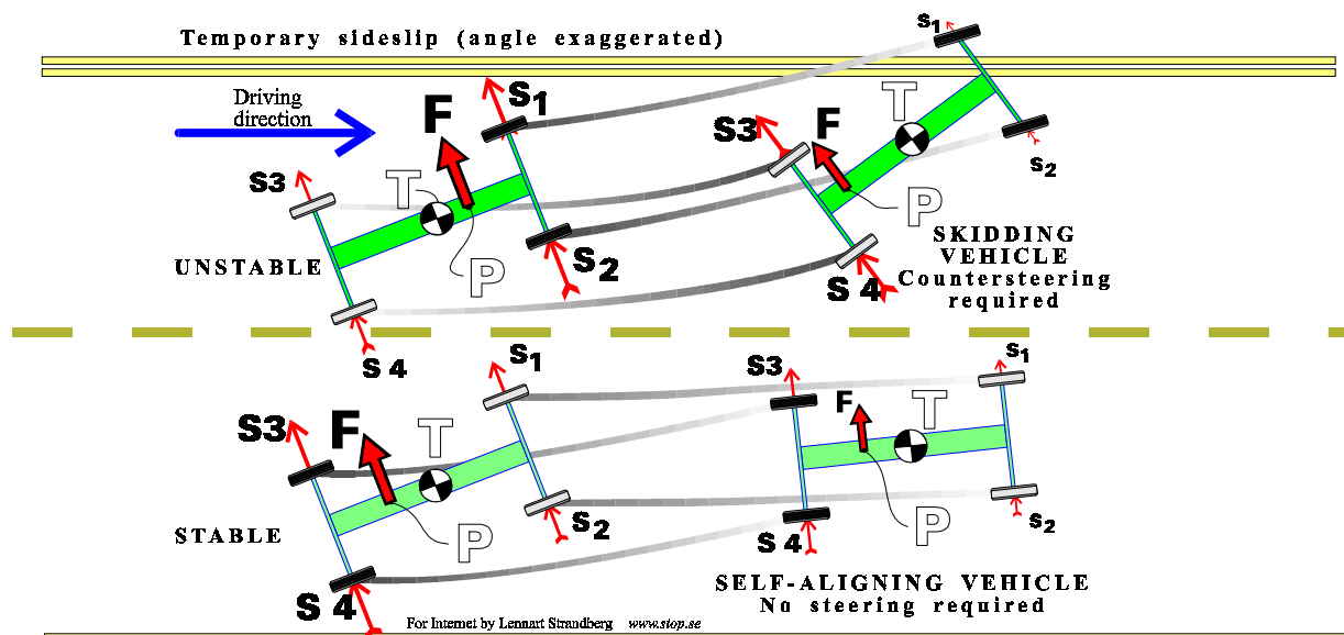
Fig.2 Simplified illustration of how stability may be lost, if the cornering stiffness coefficient, K=S/\alpha/N (Side force per sideslip \alpha angle unit divided by Normal force), is superior at the front tyres. Figure notation: Side forces (S), their resultant (F) and the position (P) of its application point in relation to the mass centre (T).
