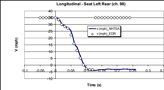
Figure 42. NHTSA Test 5578- 2006 Chevrolet Monte Carlo (with EDR time shift of -0.060s)
