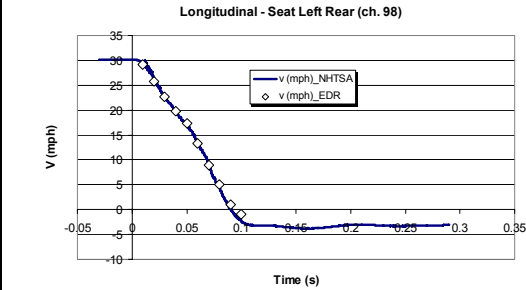
Figure 40. NHTSA Test 5213- 2004 Chevrolet Avalanche (with no EDR time shift)
