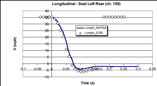
Figure 38. NHTSA Test 5250- 2005 Pontiac G6 (with EDR time shift of -0.049s)
